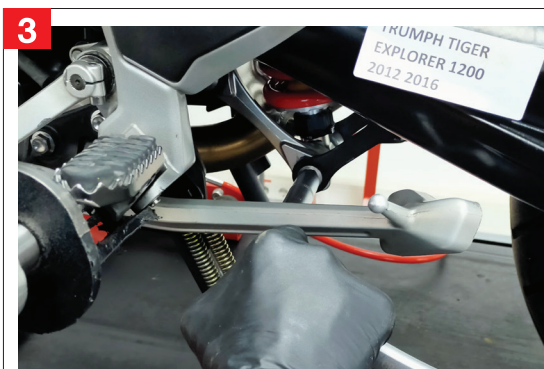
7. assemble the original bolt top and bottom
