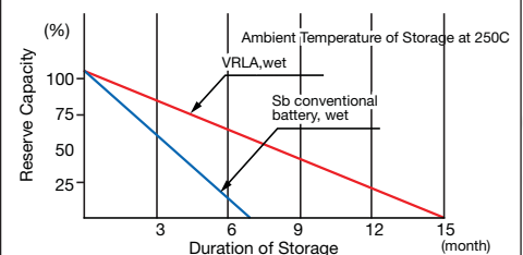
Self Discharge
